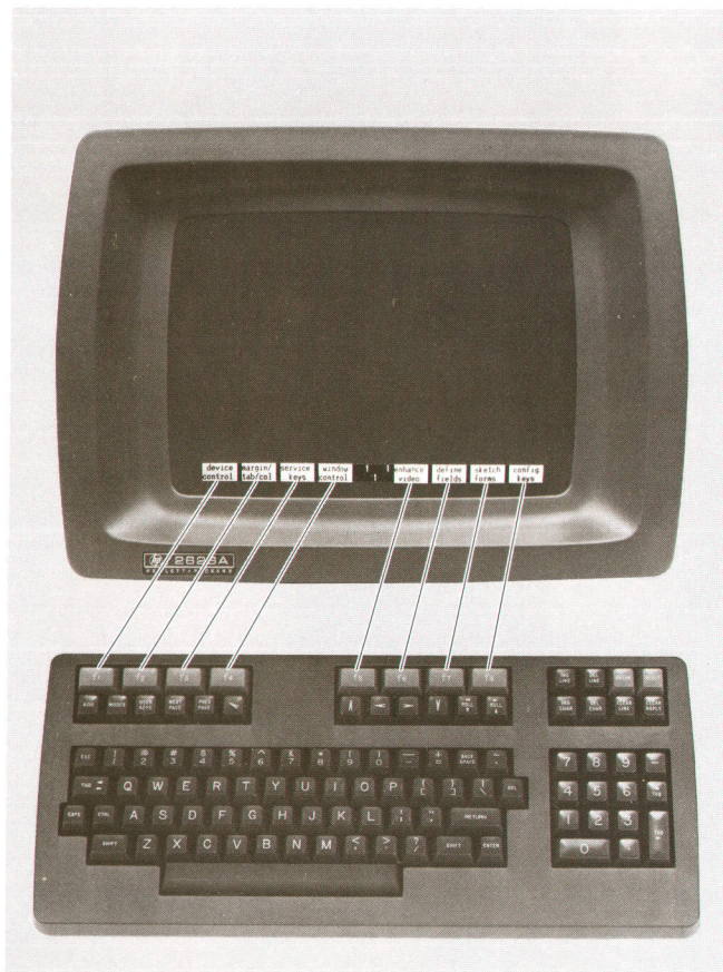
Fig. 1. The relationship between the eight softkeys and their screen labels.
