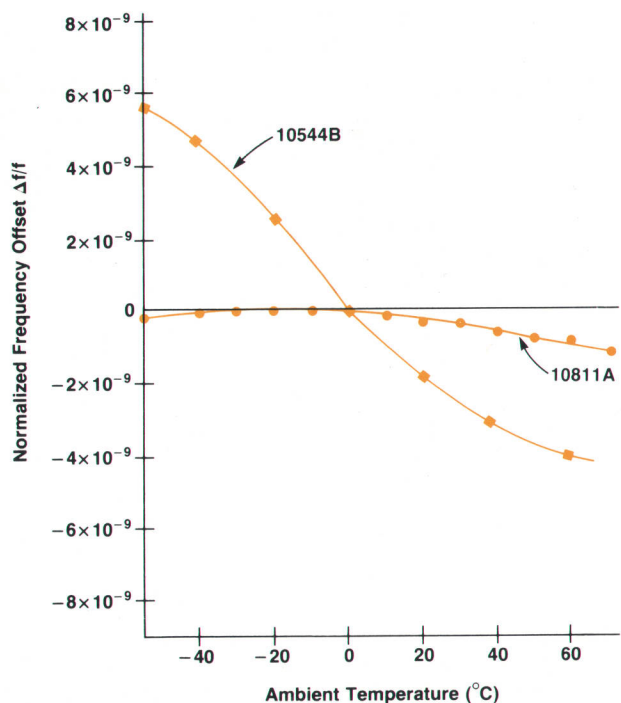
Fig. 5. The new 10811A/B Oscillator's frequency is much less sensitive to ambient temperature than the older 10544B's.
